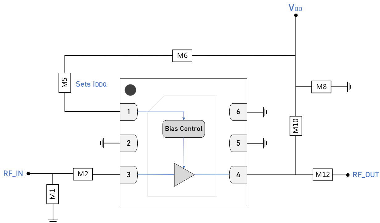
GRF2105 Standard Evaluation Board Schematic
