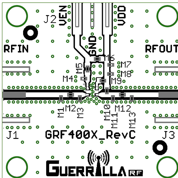
GRF2105 Evaluation Board Assembly Diagram
